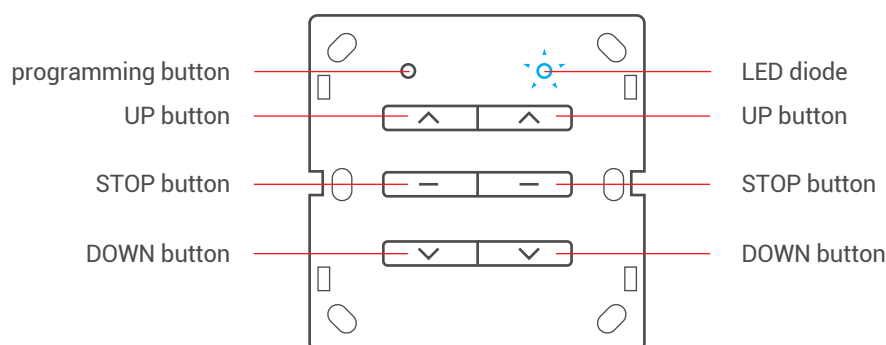
2-channel CAMELEO wall-mounted control unit (front)
