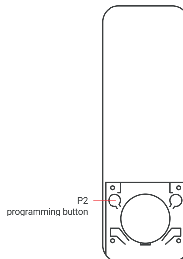
Single- or 15-channel transmitter (back)
